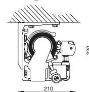
Loftmontering Ceiling installation
