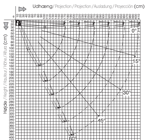
Loftmontering / Ceiling installation
